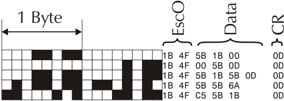
Figure 2-7 Line by Line Image Object & Hexadecimal Code with control characters
